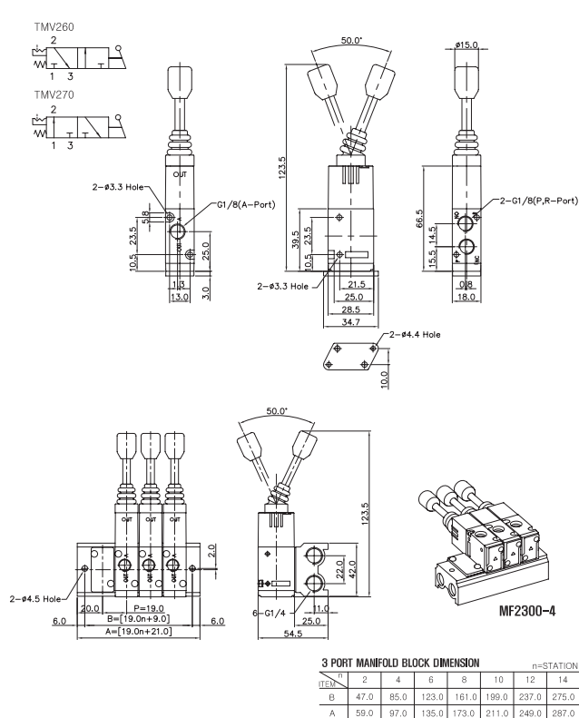
3/2-Way, Toggle Lever Manually Actuated Valve Thread-G1/4
