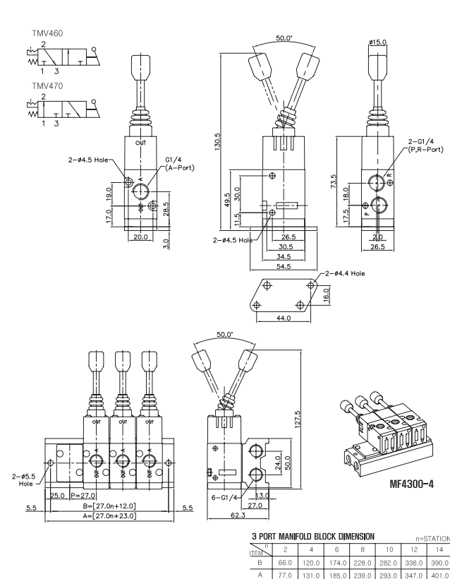
3/2-Way, Toggle Lever Manually Actuated Valve Thread-G1/4
